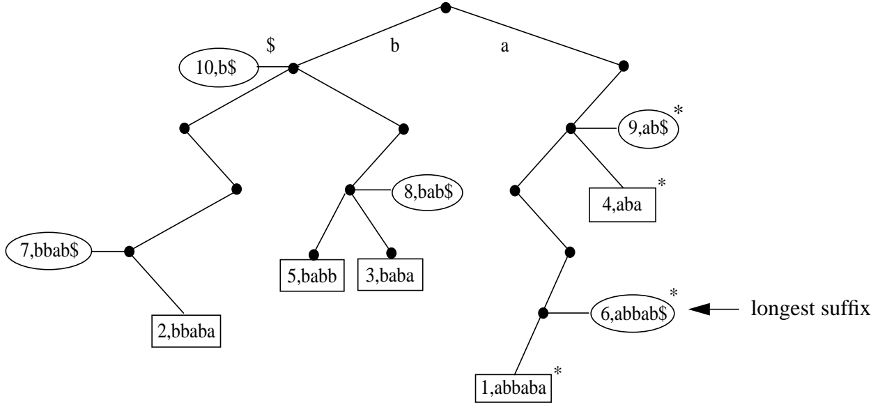
Figure 1: The suffix tree of \text{abbababbab}\$ with its longest suffix and markers shown (denoted by asterisks).
